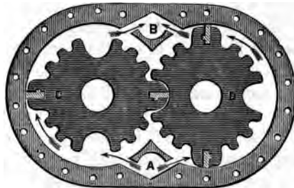
FIG. 123.—Rotary Steam-Engine.
